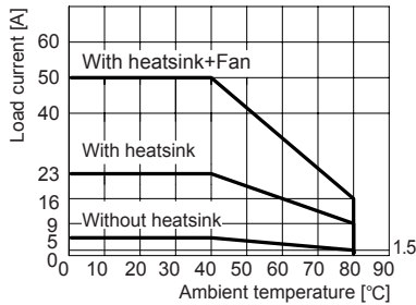
◎ SR(H)2/SR(H)3-1275/1475/1475R/2475
